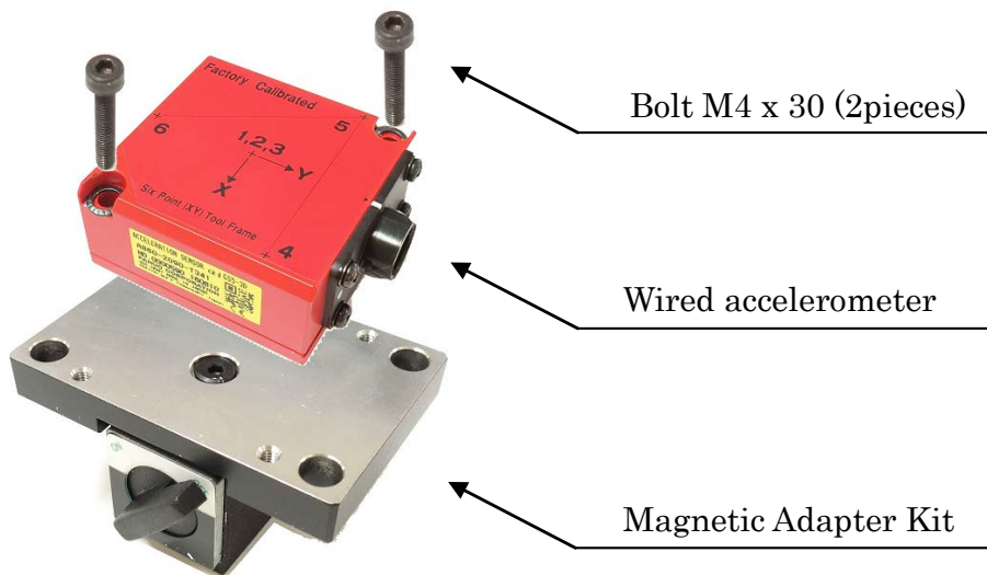
Fig. 2.1.1 (c) Magnetic adapter kit for wired accelerometer
