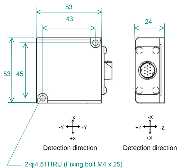
Fig. 2.1.1 (a) Dimensions of the wired accelerometer
